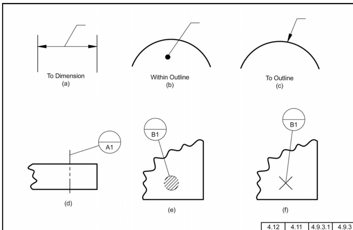
Fig. 4-9 Termination of Leaders
