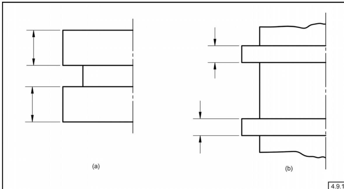
Fig. 4-7 Arrowhead Placement on Dimension Lines
