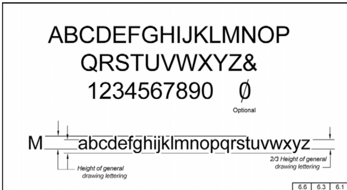
Fig. 6-2 Vertical Letters
