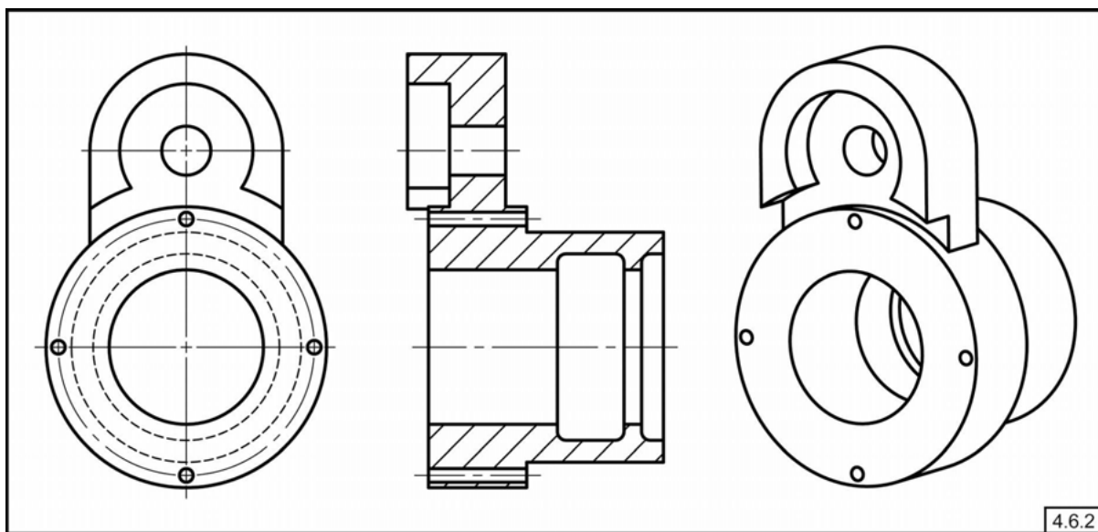
Fig. 4-5 Full Section
