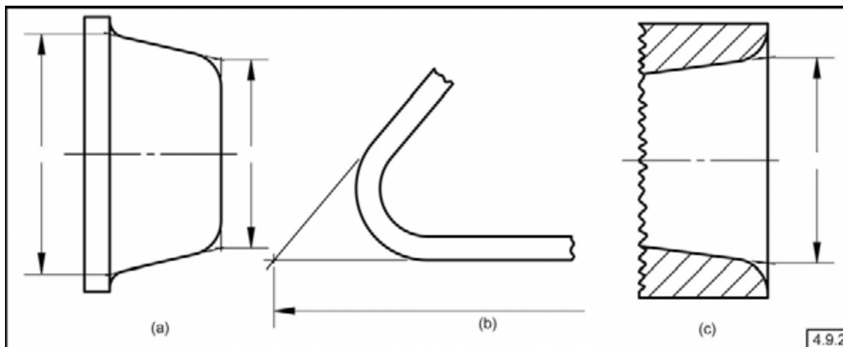
Fig. 4-8 Special Applications of Extension Lines
